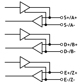
RS422 Line Transceiver
