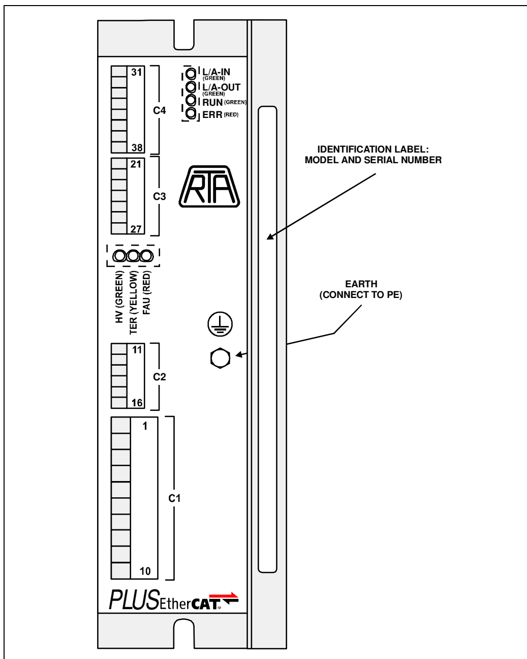
Fig. 5 – Alert led and connectors.
