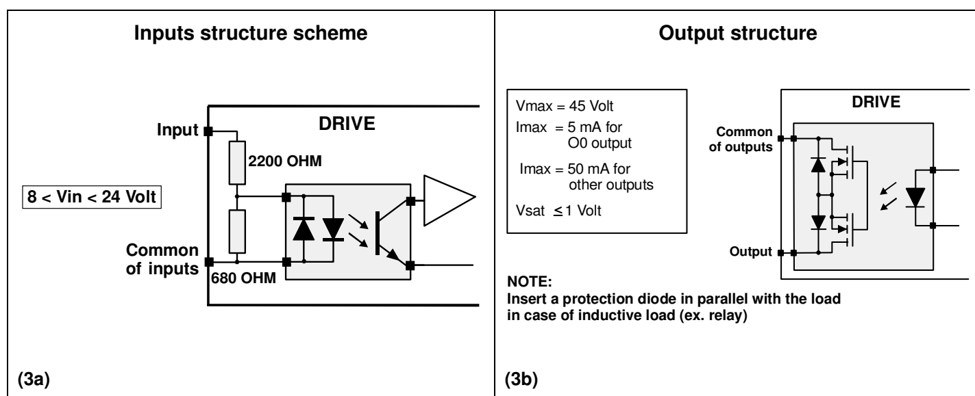
Fig. 3 – Inputs and outputs scheme.
