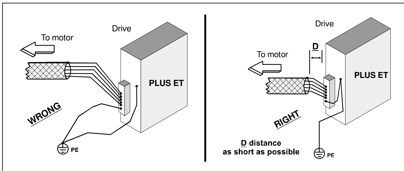
Fig. 12 - Shielded connection at drive side.
