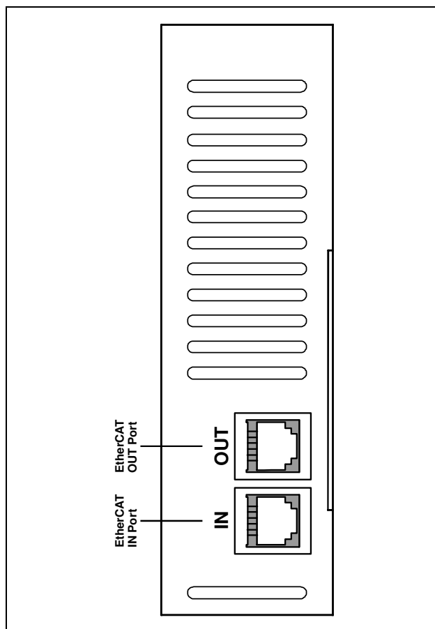
Fig. 5 – EtherCAT connectors (PLUS ET series drives high side view).
