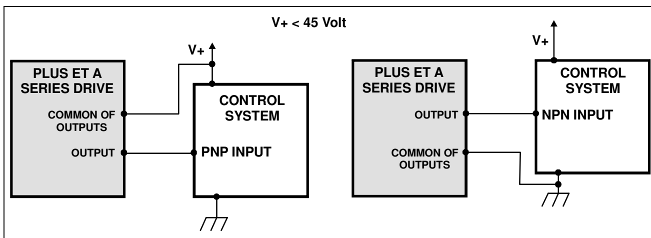
Fig. 7 – Electric connection between a PLUS ET A logic output and an input of a control system operating at V+ voltage.
