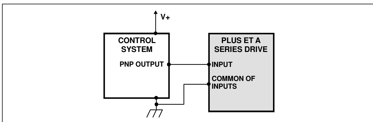
Fig. 10 - Driving a PLUS ET A logic input from a control system with a PNP output.
