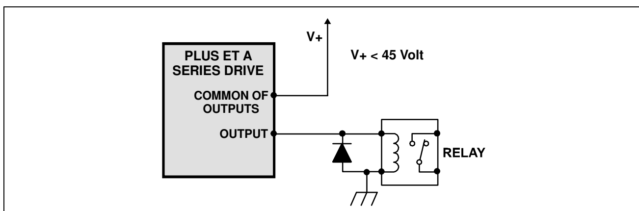
Fig. 8 - Driving a micro-relay by means of a PLUS ET A logic output.
