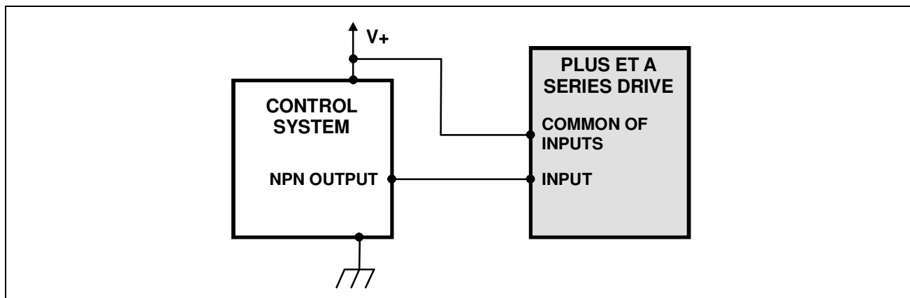
Fig. 9 - Driving a PLUS ET A logic input from a control system with a NPN open collector output.
