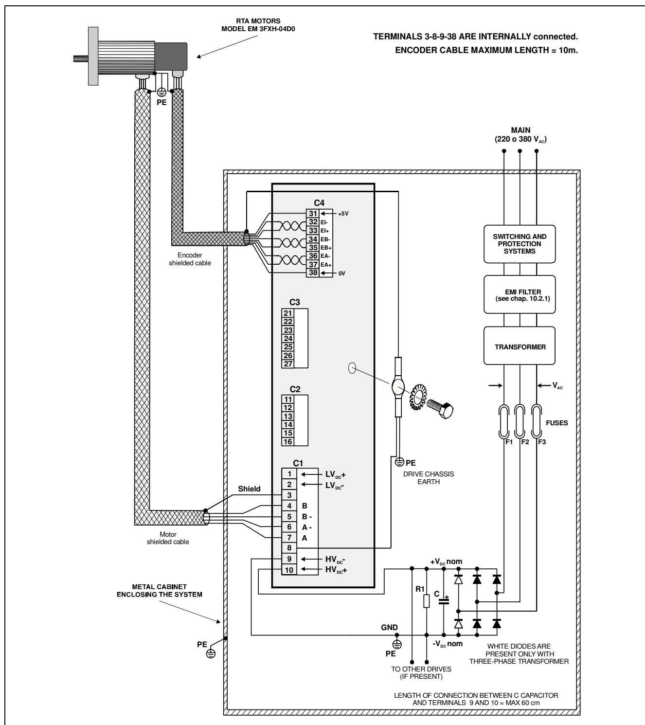
Fig. 6 – Drive external connections scheme.
