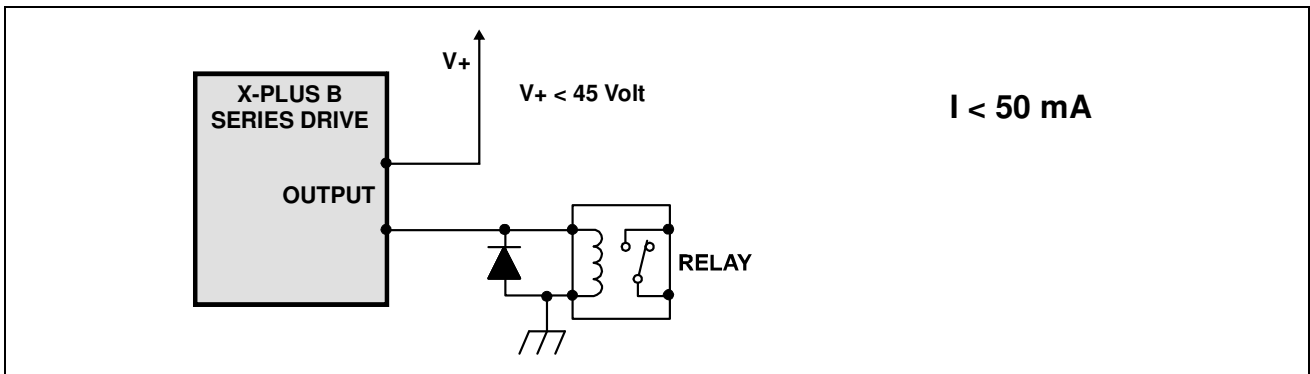
Fig. 7 Driving a micro-relay by means of a X-PLUS B logic output.
