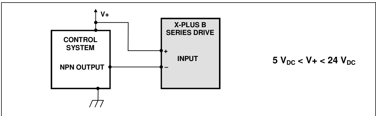
Fig. 8 Driving a X-PLUS B logic input from a control system with a NPN open collector output.
