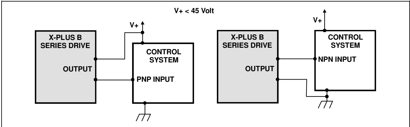
Fig. 6 Interfacing a X-PLUS B logic output and an input of a control system operating at V_+ voltage.
