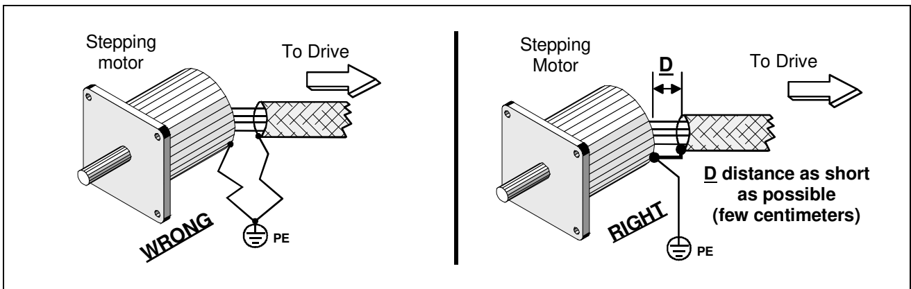
Fig. 1210 Shielded connection at stepping motor side.
