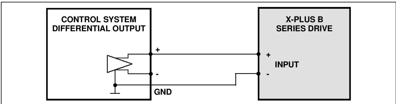
Fig. 11 - Connection example with control system with DIFFERENTIAL output (or LINE DRIVER or RS422).
