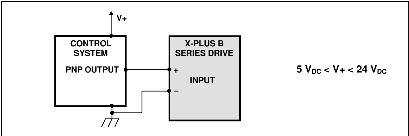
Fig. 9 Driving a X-PLUS B logic input from a control system with a PNP output.
