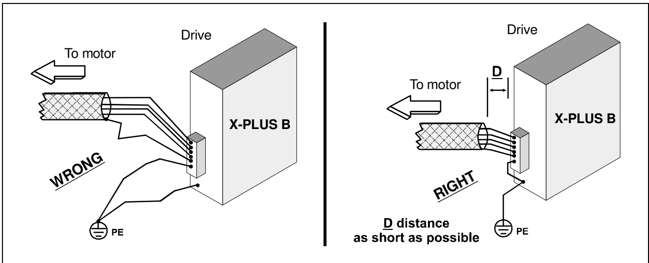
Fig. 13 Shielded connection at drive side.
