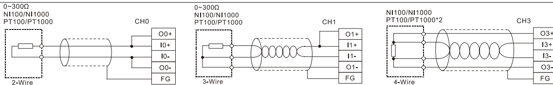
RTD 2/3/4-WIRE
