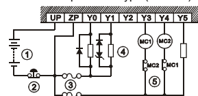
Transistor output - PNP type (SX211S):
