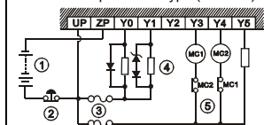
Transistor output - NPN type (SX211T):
