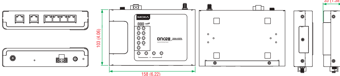
Top & Bottom View
