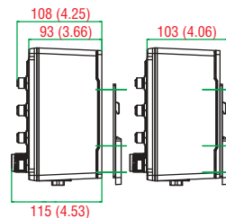
Side View (including DIN-Rail)
