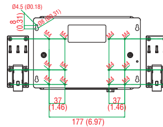
DIN-Rail Mounting Kit
