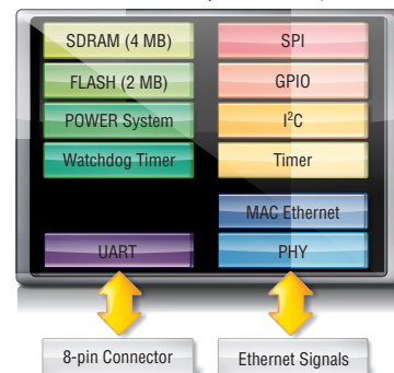
MOXA MiiNe (196-pin CPU)
