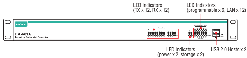
DA-681A-DPP & DA-681A-DPP-T
