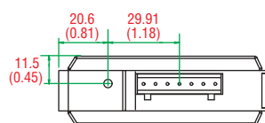
NPort IA5150-M-SC NPort IA5150-S-SC NPort IA5150I-M-SC NPort IA5150I-S-SC
