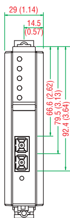
NPort IA5150 NPort IA5150I NPort IA5150-M-SC NPort IA5150-S-SC NPort IA5150I-M-SC NPort IA5150I-S-SC
