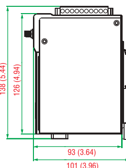
Left & Right Side View
