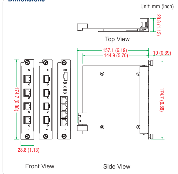
IM-G7000A-4GSFP
