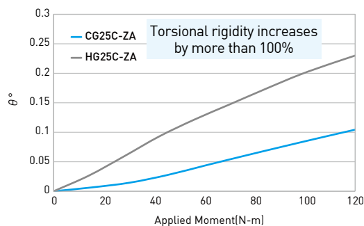
Rigidity Test
